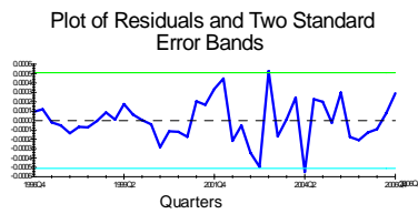
ARDL(4,0,0,0)
